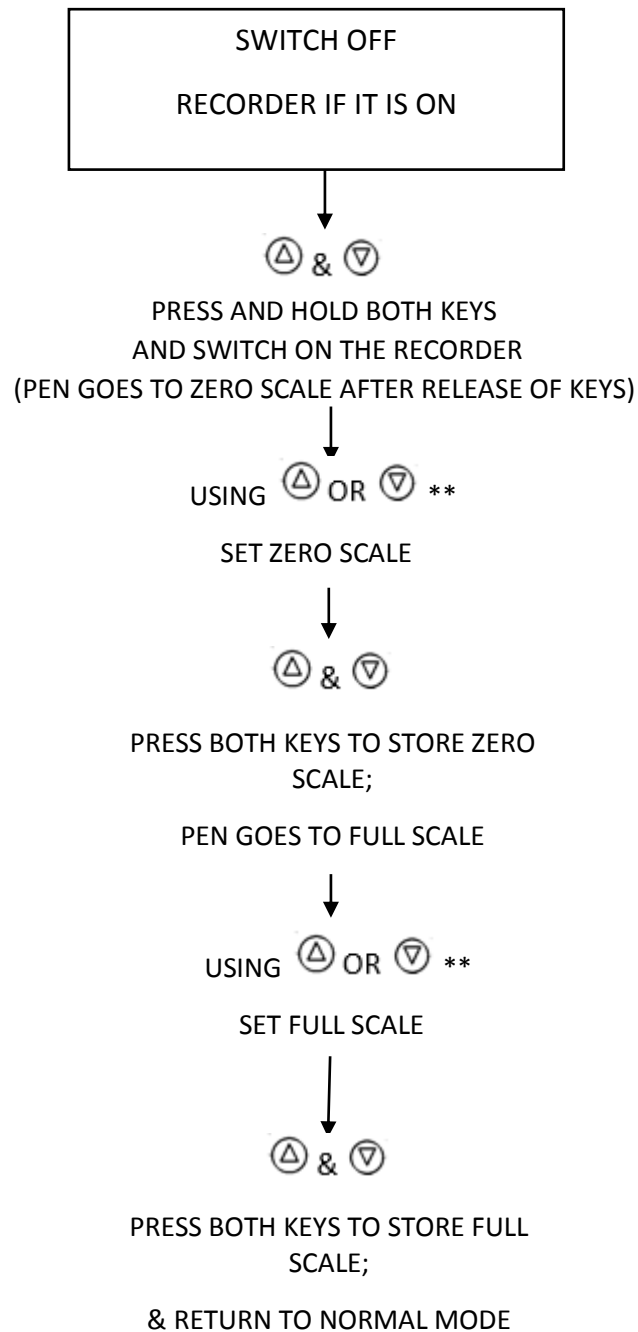
Figure 15- MECHANICAL CALIBRATION
