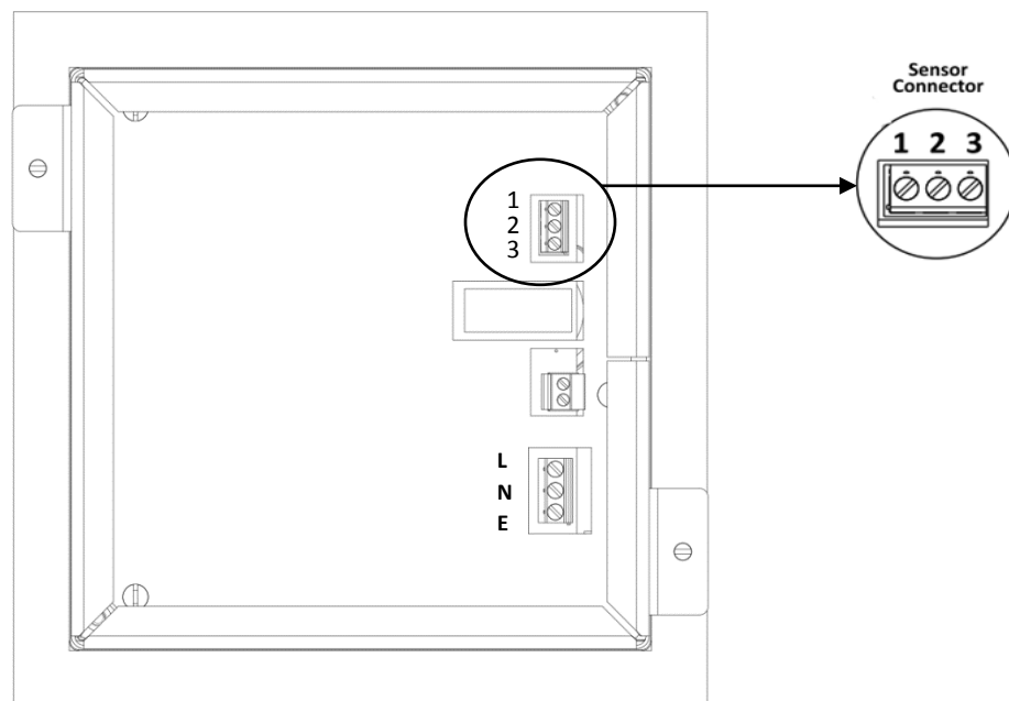
Figure 7- SENSOR WIRING
